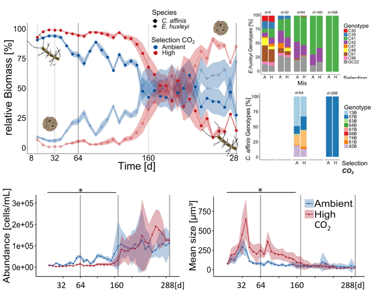
Figure 2: Upper row: Species and genotype sorting in response to two different \text{CO}_2 treatments over 288 days of selection (after Listmann et al. 2020). Lower row: Total community change in abundance and mean size in response to \text{CO}_2 (after Hattich et al. in preparation).
