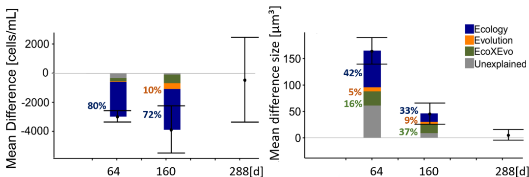
Figure 1: The relative importance of inter- (Ecology) and intraspecific (Evolution) compositional changes and their interaction for the total phytoplankton change in abundance and mean size over 288 days (corresponding to approximately 180 generations).
