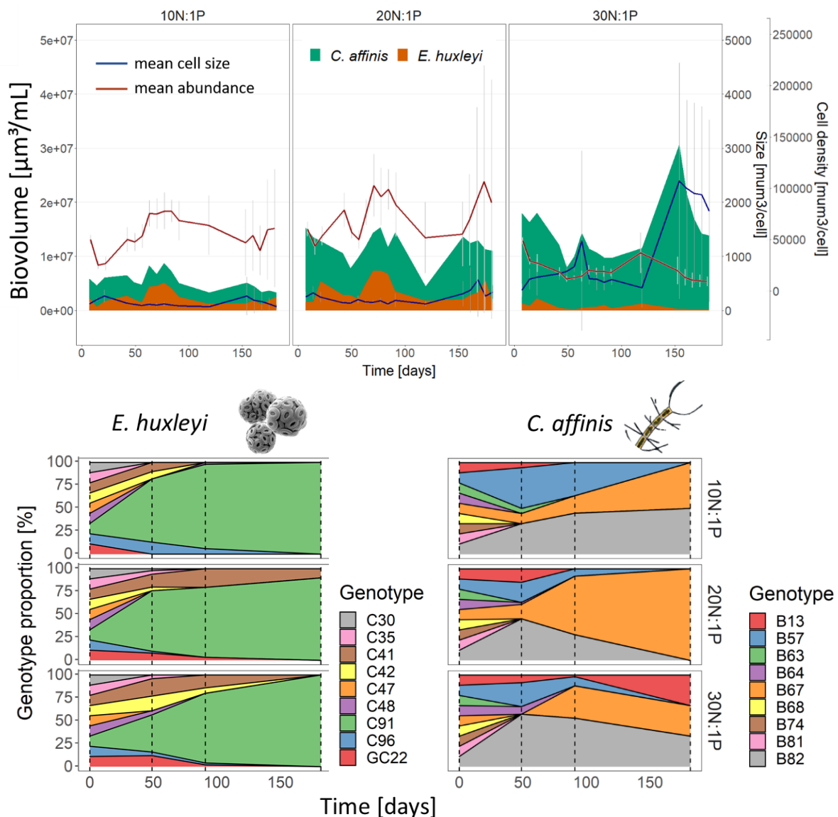
Figure 3: Upper graphs: Total biomass, mean abundance and size, species composition in response to nutrient regimes over 180 d which approximately corresponds to 130 phytoplankton generations. Lower graphs: Genotype sorting of the two species in response to nutrient regime
