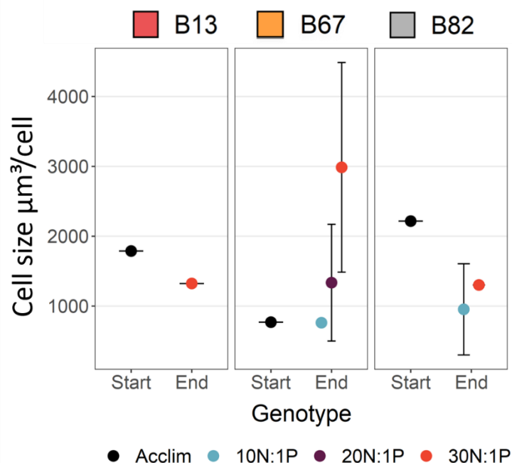
Figure 4: Size plasticity of remaining C. affinis genotypes over the nutrient treatments at the end of the long-term experiment compared to mean size at the onset.
